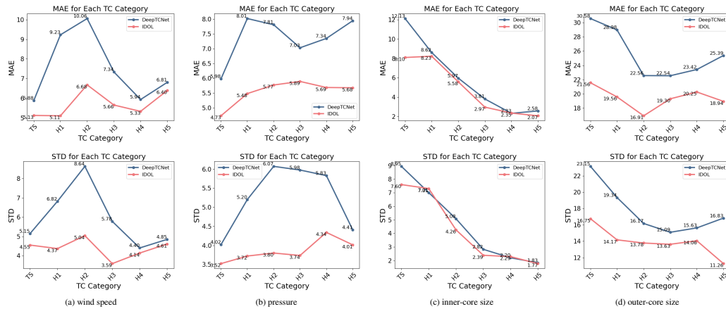
Figure 9: Visualization of estimation results across TC categories on our PDTc dataset. From left to right: estimated wind speed, pressure, inner-core size, and outer-core size.
