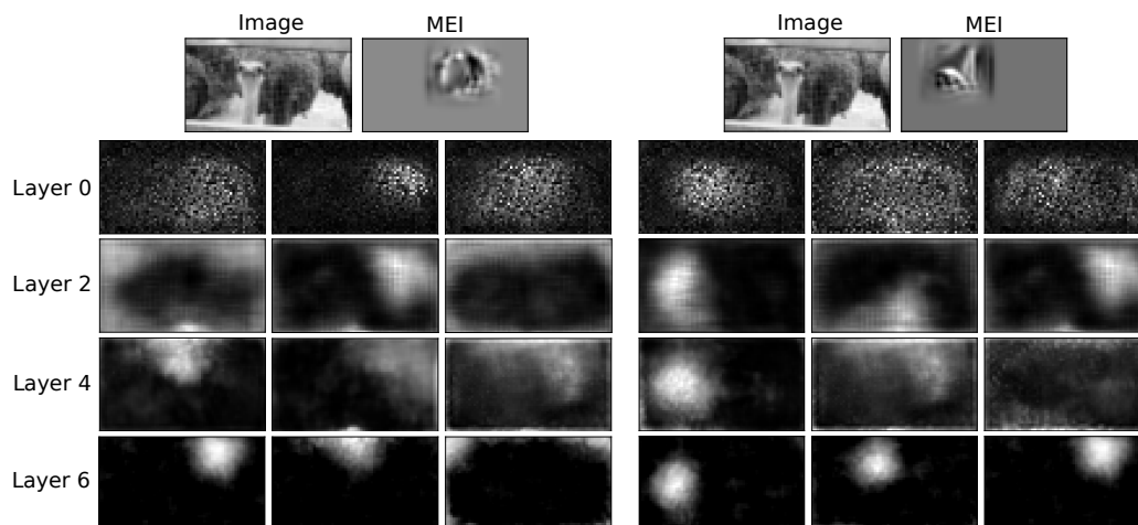
Figure 10: Input images, MEIs, and visual concepts with the highest activation gain for two example neurons from the BRAINREADER dataset. For each MEIcoder core layer and neuron, the top three concepts (NMF features) are shown, ordered by the increase in the corresponding feature coefficient between a forward pass with the neuron's response set to zero and one with it set to 10 \cdot p_{.99} , where p_{.99} denotes the neuron's 99th activation percentile in the dataset.
