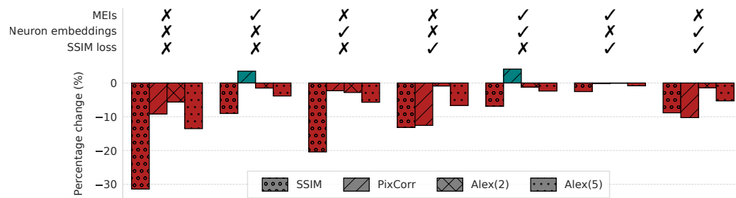
Figure 4: Ablation study on sub-components of MEIcoder. The percentage (y-axis) is calculated with respect to a setting with no ablations. Reported values are the average across the three datasets.
