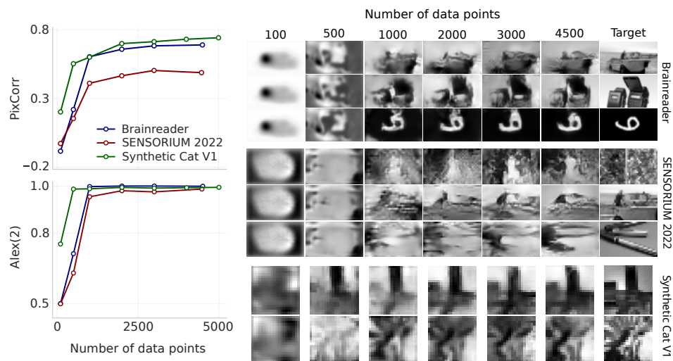
Figure 7: Relationship between MEIcoder's performance and the number of training data points.
