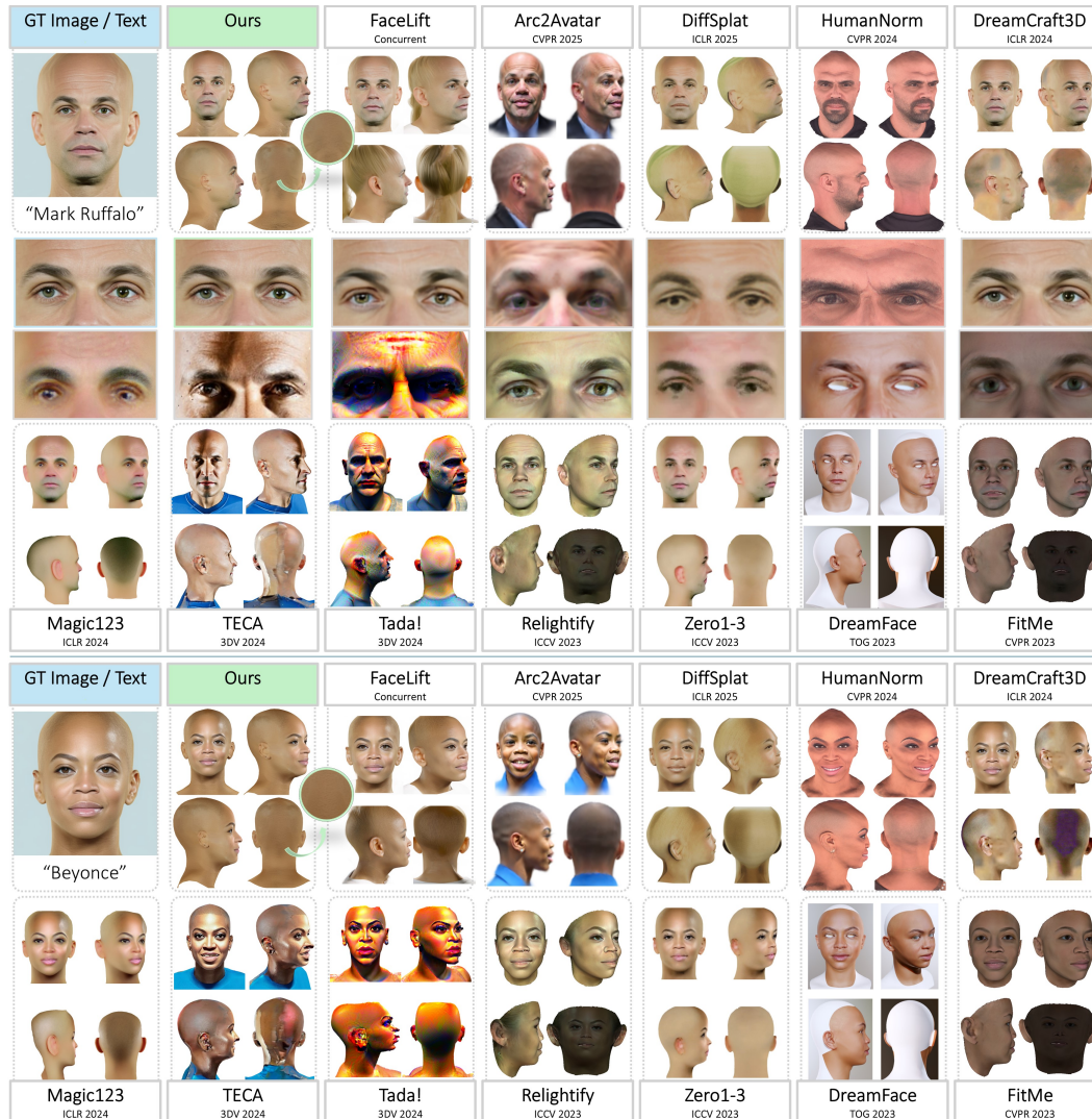
Figure 3: Qualitative Comparison with State-of-the-Art: We compare HairFree against recent 3D avatar techniques—FaceLift [41], Arc2Avatar [18], DiffSplat [38], HumanNorm [21], Dream-Craft3D [60], Magic123 [50], TECA [69], TADA! [36], Relightify! [46], Zero123-XL [39], Dream-Face [70], and FitMe [29]—on “Mark Ruffalo” and “Beyonce” with explicit bald-head constraints. HairFree delivers the most accurate 360° head shapes, realistic textures, and uniform lighting.
