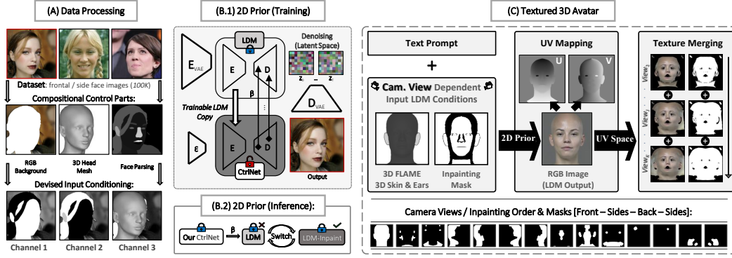
Figure 2: System Overview: (A) Data Processing : Estimate face parsing, 3D head mesh, and remove the foreground to form compositional inputs. (B.1) Training Prior : Fine-tune an LDM via ControlNet using these inputs and a generic “face” prompt. (B.2) Inference Prior : Swap in a generic LDM-Inpainting prior. (C) Texture Generation : Generate a frontal view, map to UV space, iteratively render “seen” and inpaint “unseen” regions while moving the camera, building a full 360° texture.
