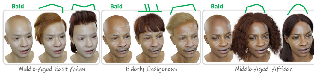
Figure 1: HairFree is a hybrid 2D/3D neural rendering method that synthesizes diverse, high-fidelity 360° bald human head textures given a 3D head mesh and a textual description. The generated bald textures (columns 1, 4, 7) seamlessly integrate into classical graphics pipelines, allowing compatibility with any 3D hairstyle—regardless of hairline type (in green)—in a fully compositional manner.
