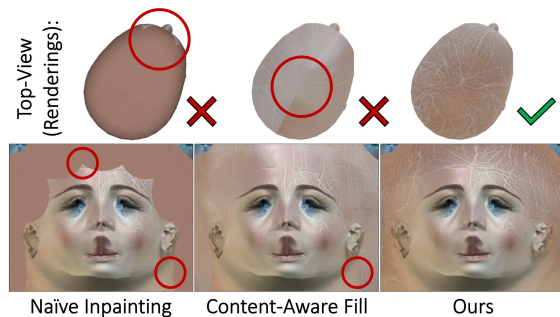
Figure 8: Comparisons: Inpainting in UV Space.
