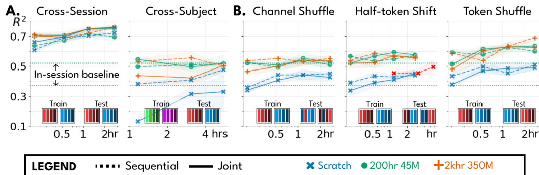
Figure 12. A replication of Fig. 4A/B, but showing results for both sequential and joint fine-tuning in each setting, and on multiple fine-tuning data scales. As before, each model here tunes with some data from other settings (e.g. cross-subject data for the cross-subject panel), and a fixed amount of data on the test session. Sequential tuning first tunes on other-setting data, and then tunes on test session data. Joint tuning uses all data at once. In Fig. 4A/B, we only showed the better choice for each panel, i.e. we showed joint tuning for cross-session data, and sequential tuning for the other settings. In addition, we overlay how the cross-subject tuned models perform when applied to half-token shifted test data, confirming that subject and session data transfer similarly to shifted test data. Shading shows the standard deviation on 3 model seeds. In-session baseline refers to the no-intermediate tuning setting in Fig. 4B.
