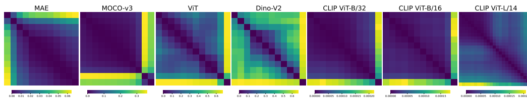
Figure M.19: Layer-wise Jensen-Shannon Divergence (JSD) between predicted class probabilities across different architectures. Each heatmap corresponds to a specific model and illustrates the pairwise JSD between layers. Color intensity reflects the degree of divergence, with brighter values indicating greater dissimilarity in output distributions. Note that each subplot uses its own color scale to emphasize internal variation within each architecture.
