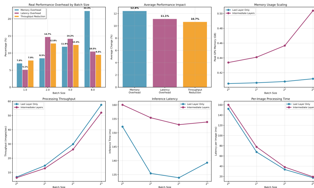
Figure L.13: Computational cost comparison for CLIP RN50x4 using intermediate layers versus last-layer only inference.
