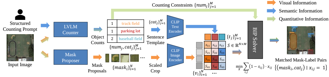
Figure 3: The InstructSAM framework. Given an input image and a structured counting prompt, the LVLN Counter extracts target categories \{cat_j\} (semantic info) and their counts \{num_j\} (quantitative info). Concurrently, the Mask Proposer generates mask proposals \{mask_i\} (visual info). A CLIP model computes the similarity matrix S between mask embeddings (from scaled crops) \{v_i\} and category embeddings \{t_j\} . Finally, the Binary Integer Programming (BIP) Solver optimally assigns categories to masks by maximizing summed similarity, subject to the counting constraints, yielding the final recognition results.
