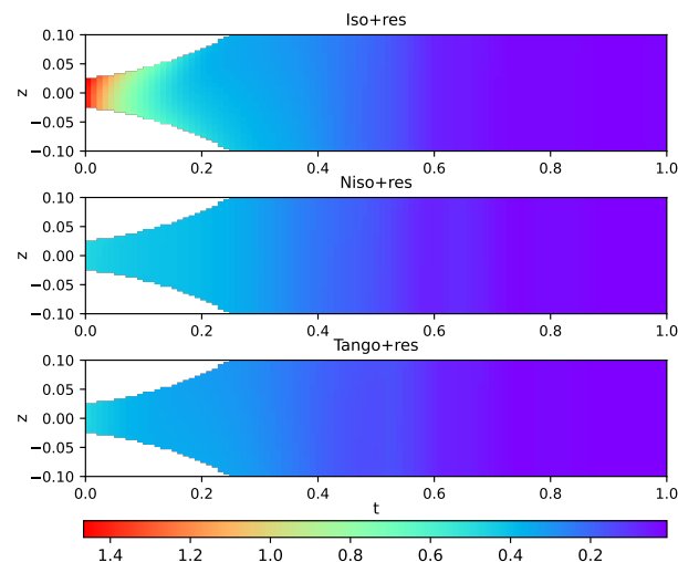
Figure 1: The average error of the tangential component of the learned score function in the x - y plane, along the z -axis and t -axis, with \sigma_{\min} = 0.01 . From top to bottom, the plots correspond to the vanilla algorithm (Iso-DM), our proposed Niso-DM and Tango-DM, all using the rescaling technique.
