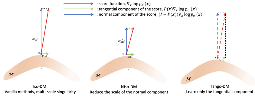
Figure 2: Schematic diagrams of the vanilla method (left), our proposed Niso-DM (middle), and tango-DM (right).
