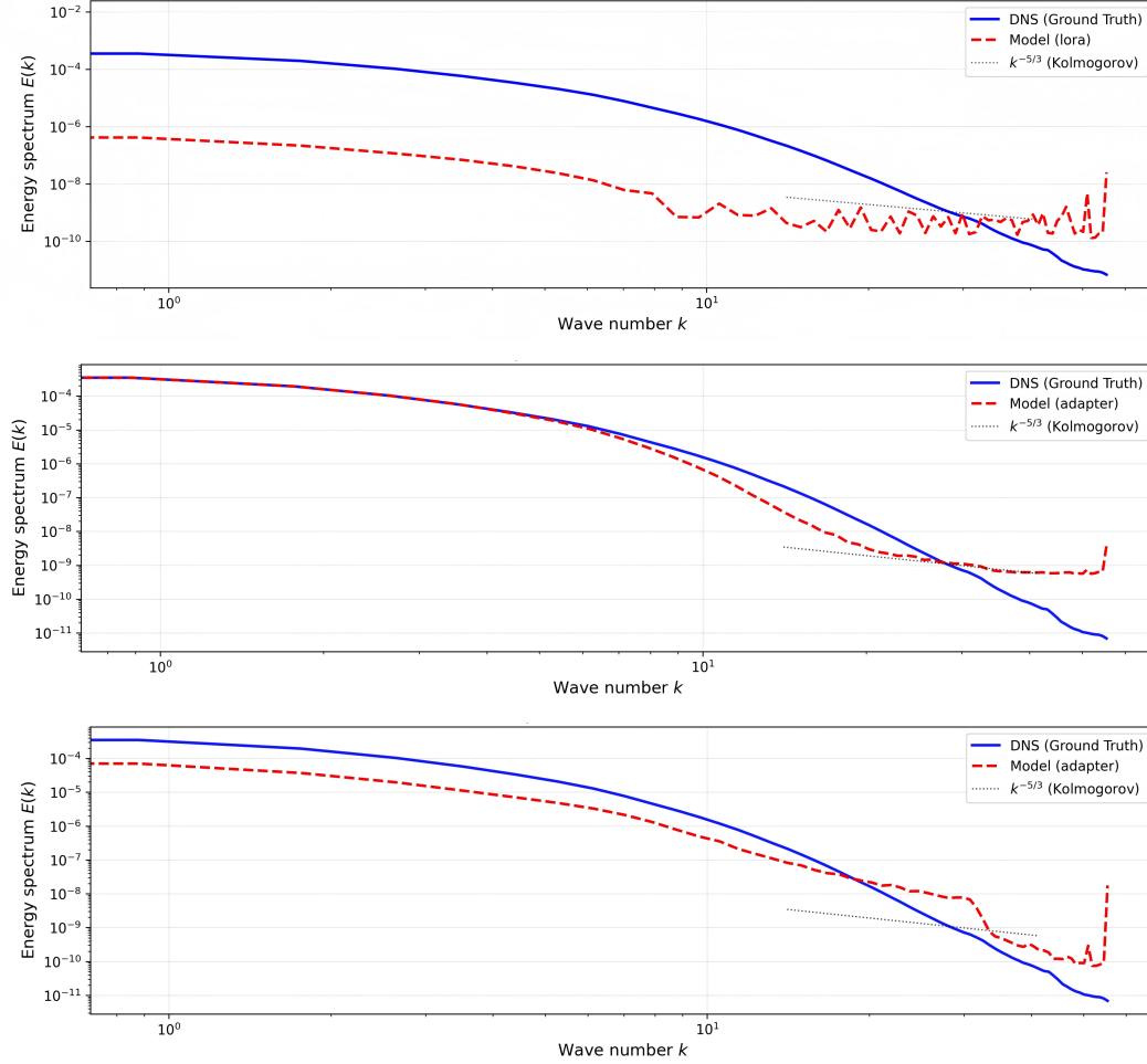
Figure 8: Energy spectra E(k) on logarithmic axes for three PEFT methods, each compared to DNS (blue) and a k^{-5/3} reference slope (gray). From top to bottom: LoRA, F-Adapter (Ours), and Vanilla Adapter. F-Adapter follows the DNS spectrum more closely across a broad range of wavenumbers, while Vanilla Adapter shows a deficit at mid-to-high k and LoRA substantially underestimates energy with noisy behavior at large k .
