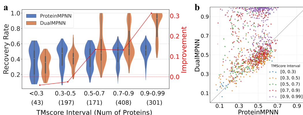
Figure 2: Impact of template quality on sequence recovery rate. (a) Violin plot comparing sequence recovery rates of DualMPNN and ProteinMPNN across distinct TM-score intervals on the CATH test set. (b) Scatter plot of per-protein recovery rates, colored by TM-score intervals. Points above the dashed parity line ( y = x ) highlight instances where DualMPNN outperforms the baseline, particularly for high-quality templates (TM-score > 0.5).
