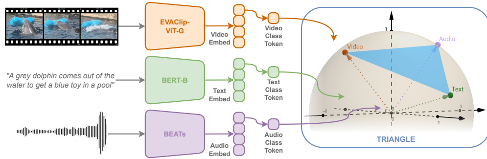
Figure 2: TRIANGLE builds the high-dimensional space spanned by the embeddings generated by the encoders. The embedding vectors of the three modalities lie within a unit hypersphere, where they form a triangle. The area of this triangle is an unambiguous measure of their alignment.
