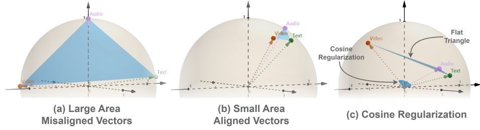
Figure 3: (a-b)TRIANGLE area as a measure of similarity. Misaligned vectors, large area (a); Aligned vectors, small area (b). (c) In the case of a flat triangle, we apply the cosine regularization, bringing the alignment information between the two modalities on which the downstream task is about. In the example of video-text retrieval, we regularize with the cosine between video and text.
