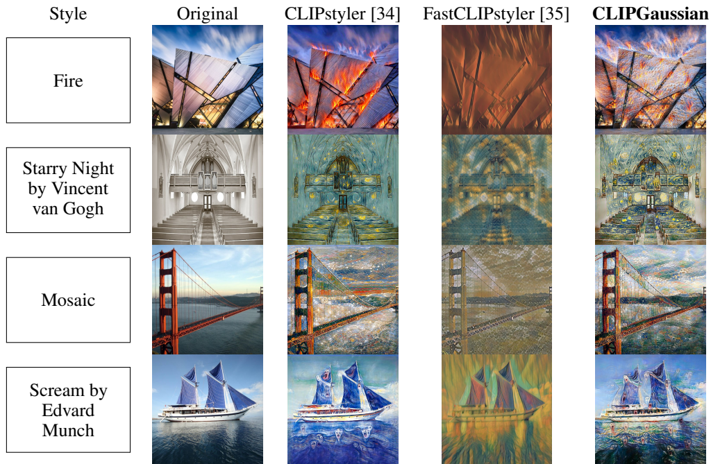
Figure 34: Comparison of image style transfer using text condition.
