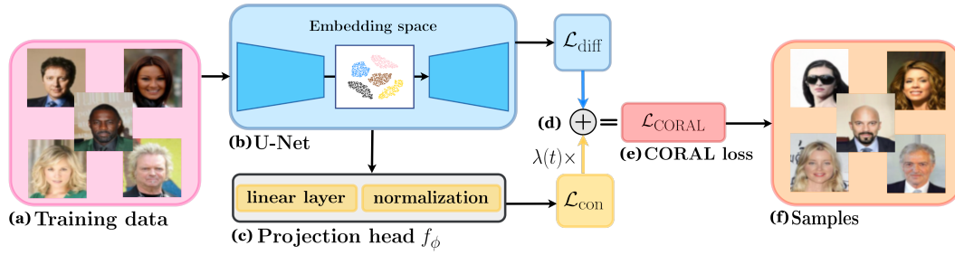
Figure 2: CORAL architecture and workflow on CelebA-5. (a) The five-class CelebA-5 training data is input to the U-Net architecture. (b) Denoising U-Net. The white inset shows an actual t-SNE visualization of the U-Net latent representations due to CORAL. (c) CORAL’s addition to the standard DDPM architecture: a projection head MLP consisting of a single dense layer followed by normalization. (d) The output from the U-Net and the projection head are used to compute the corresponding diffusion and contrastive losses. (e) The contrastive loss is scaled by a time-dependent weighting function, \lambda(t) , and added to the standard diffusion loss to obtain the CORAL loss. (f) Samples are obtained from a trained CORAL model.
