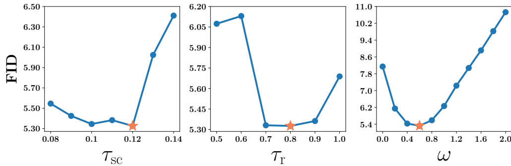
Figure 8: Effect of regularization hyperparameters and guidance scales on FID. From left to right: FID vs \tau_{SC} , FID vs \tau_r , and FID vs \omega for the CIFAR10-LT dataset. Coral stars mark the lowest FID achieved for each hyperparameter.
