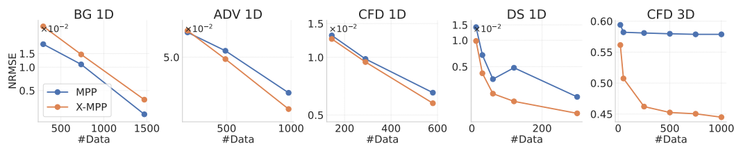
Figure 5: Test NRMSE of finetuning on unseen dimensions (1D and 3D).
