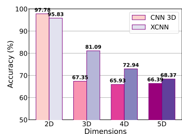
Figure 4: Accuracy on GP kernel prediction.
