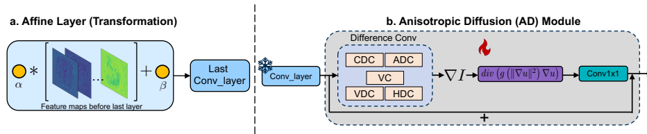
Figure 3: (a) Learnable affine transform scales feature maps by \alpha and \beta before the final layer. (b) Learnable AD module \text{flame} refines images while preserving structures, with frozen convolution \text{star} .
