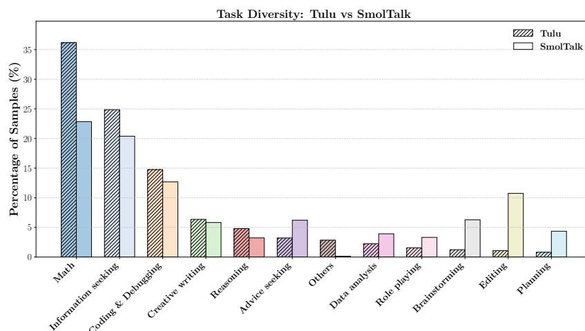
Figure 2: Task diversity in Tulu and SmolTalk as annotated by Magpie. Bars show the fraction of each dataset devoted to different tasks (e.g., math, coding/debugging). Tulu is dominated by structured, code-centric, and mathematical prompts, whereas SmolTalk features a substantial amount of conversational tasks such as editing, information seeking, and brainstorming, alongside math.
