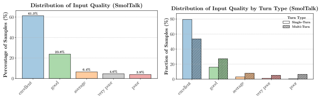
(a) Overall input quality distribution for SmolTalk: most samples (over 85%) are of “excellent” or “good” quality, indicating even stricter quality controls during dataset curation. (b) Input quality distribution by turn type for SmolTalk: most ST and MT samples are of “excellent” or “good” quality, with significantly smaller portions for “average”, “poor”, and “very poor”.
