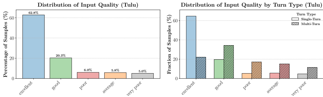
(a) Overall input quality distribution for Tulu: most samples (over 80%) are of “excellent” or “good” quality, indicating rigorous quality controls during curation. (b) Input quality distribution by turn type for Tulu: most ST samples are of “excellent” quality while most MT samples are of “good” quality, followed by “excellent”.
