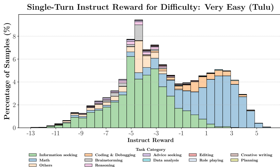
(a) Single-turn instruct reward distribution for very easy samples in Tulu.
