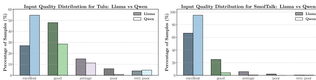
(a) Input quality distribution for a 30k stratified subset of Tulu using Llama and Qwen as Magpie annotators. Qwen strongly favors the excellent label, while Llama offers a more realistic spread.
