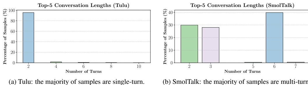
Figure 11: Distribution of the top-5 conversation lengths. Tulu is overwhelmingly single-turn, whereas SmolTalk is predominantly multi-turn, albeit with a substantial single-turn segment.
