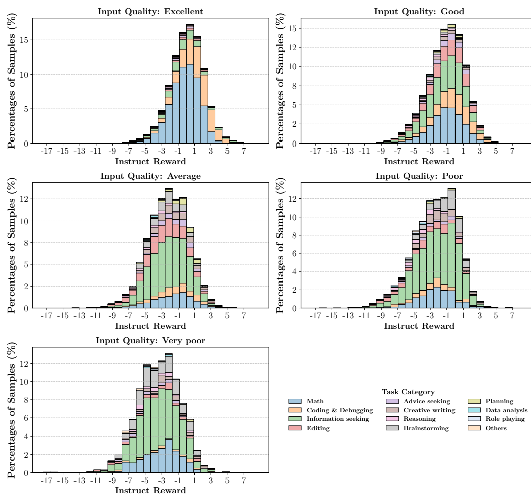
Figure 23: Distribution of single-turn instruct reward scores by input quality label in the SmolTalk dataset. As with Tulu, higher input quality is strongly correlated with higher instruct reward, demonstrating that prompt clarity and specificity are key drivers of response quality in the single-turn setting.
