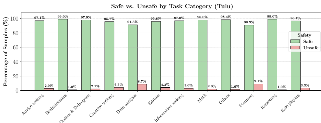
Figure 40: Distribution of safe and unsafe samples by task category in the Tulu dataset. Unsafe samples are rare and show no meaningful concentration in any specific category.
