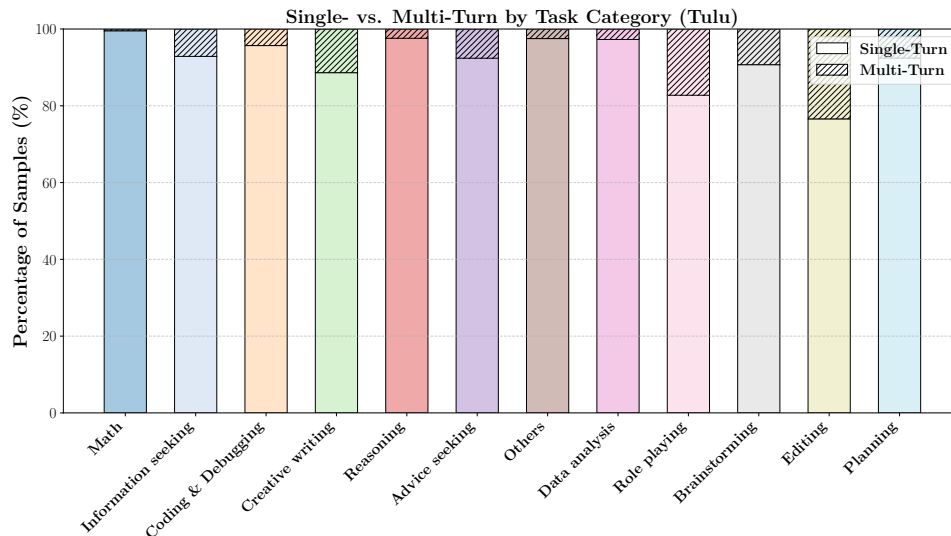
Figure 12: Turn type distribution in Tulu by Magpie task category. Most categories are dominated by single-turn (ST) samples, reflecting the dataset's focus on concise, one-shot interactions.
