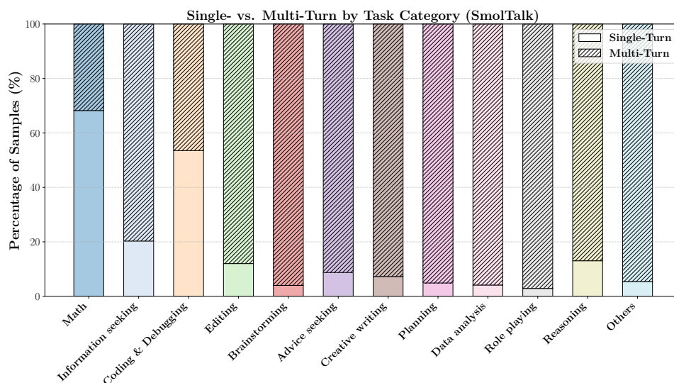
Figure 13: Turn type distribution in SmolTalk by Magpie task category. Most categories are dominated by multi-turn (MT) samples, consistent with the dataset’s emphasis on dialogic interaction. Math stands out with a higher proportion of single-turn, one-shot problem-solution exchanges.
