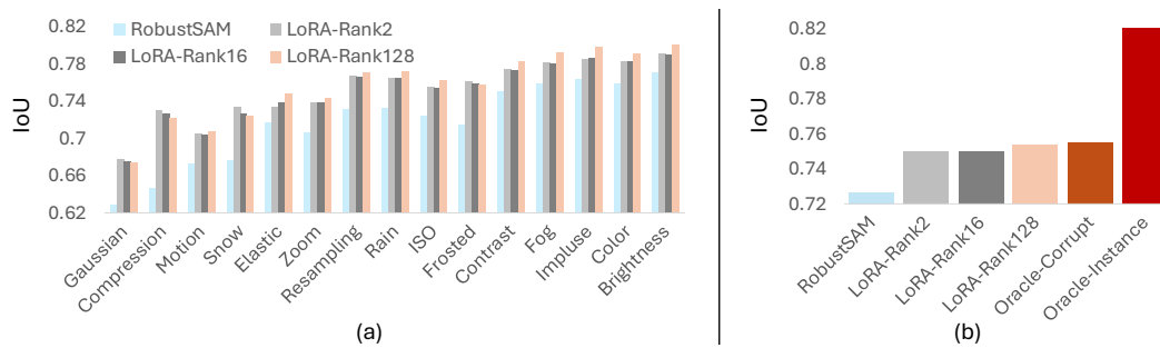
Figure 2: Impact of the rank in LoRA integrated with SAM. The models were evaluated on LVIS [15] using point prompts. (a) Performance versus rank under various corruption types. The best rank varies depending on the corruption type. (b) Comparisons of rank selection strategies. Oracle-Corrupt chooses the best rank per corruption type, while Oracle-Instance selects the best rank per image. The outstanding performance of Oracle-Instance suggests the need for input-adaptive rank manipulation.
