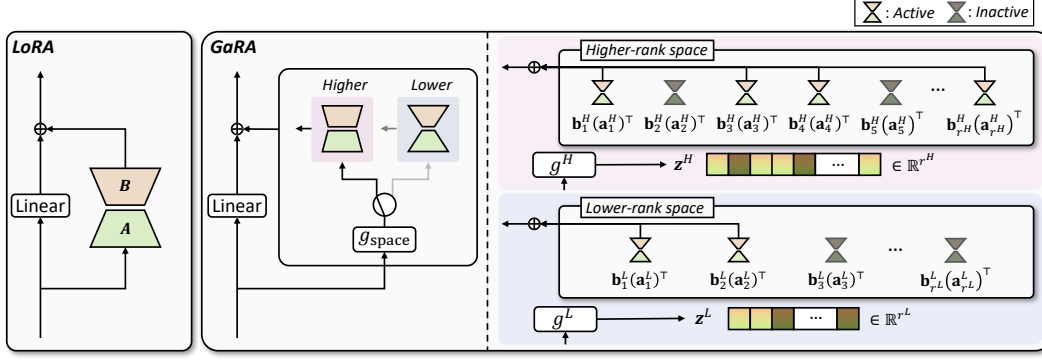
Figure 3: Adapter architecture of GaRA and comparison to LoRA. GaRA leverages hierarchical gating for both coarse and fine control over the adaptation process. First, g_{\text{space}} selects between the higher-rank and lower-rank spaces based on the input. Then, the corresponding gating module g^H or g^L predicts a binary vector \mathbf{z}^H or \mathbf{z}^L to activate a subset of (rank-1) components tailored to the input. These active components are composed to form the final update matrix for adaptation.
