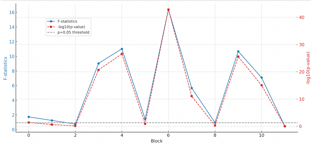
Figure a2: Statistical analysis of gated rank selection under different corruption types on MSRA10K. For each block, we compute the F-statistic and p-value (shown as -\log_{10}(p) ). A higher F-statistic and p-value below 0.05 (dashed line) indicate that the variation in activated ranks across corruption types is statistically significant.
