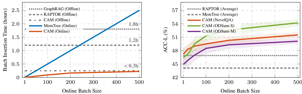
(a) Average Insertion Time vs. Online Batch Size (b) ACC-L Performance vs. Online Batch Size Figure 3: CAM’s advantages in insertion efficiency and performance stability under the online setting.
