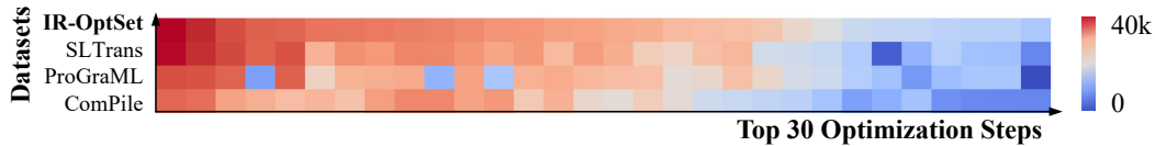
Figure 5: Heatmap analysis of the top 30 most commonly used optimization steps in LLVM 19.1.0 across four datasets. Color intensity represents the frequency of effectiveness.
