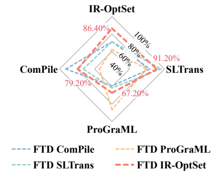
Figure 6: Generalization of 4 datasets.
