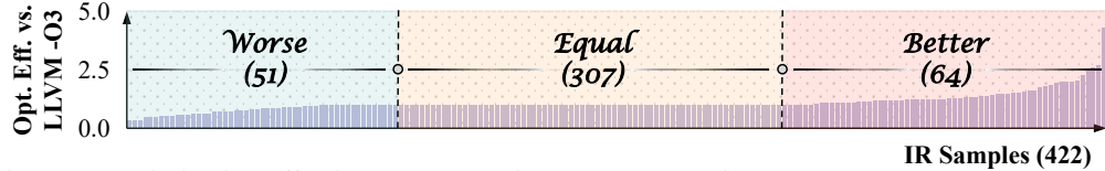
Figure 4: Optimization effectiveness comparison: LLM Compiler FTD IR-OptSet vs. LLVM -O3.
