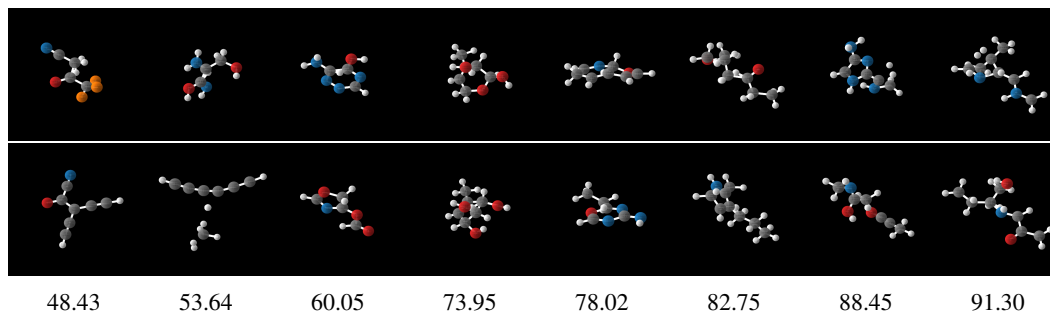
Figure 4: Qualitative visualization of controlled generated molecules for various polarizability ( \alpha ) levels. Top row is generated using end-to-end guidance with a DTO scheme and the bottom row is generated using greedy guidance.
