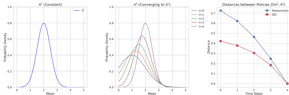
Figure 11: Jensen-Shannon distance (JSD) trends similarly to Wasserstein distance when we have continuous policies.
