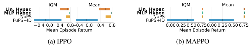
Figure 18: Performance of IPPO and MAPPO on Dispersion after 20 million timesteps. We show the Interquartile Mean (IQM) of the Mean Episode Return and the 95% Stratified Bootstrap Confidence Intervals (CI) using [1]. Hypernetworks achieve comparable performance to NoPS, while FuPS struggle with specialisation.
