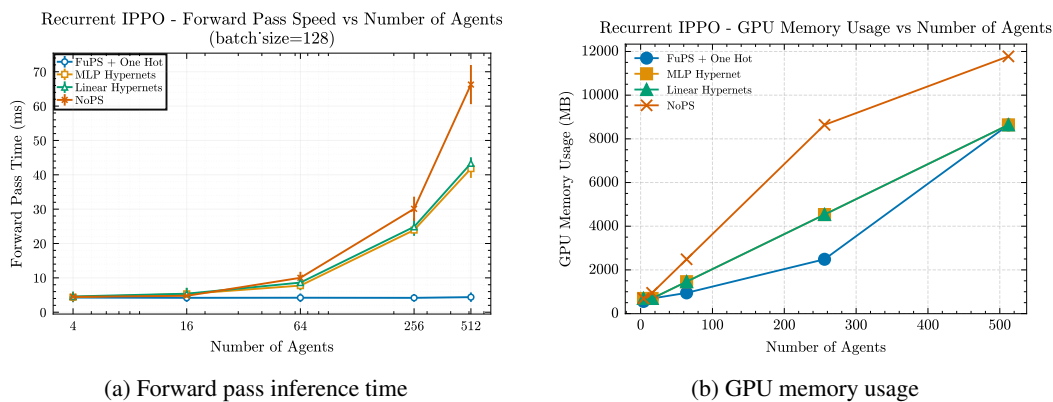
Figure 16: Computational efficiency scaling with number of agents. HyperMARL offers a balance between NoPS and FuPS. Notably, in real-world deployments, NoPS incurs additional data transfer and synchronisation costs not reflected here, further widening the efficiency gap.
