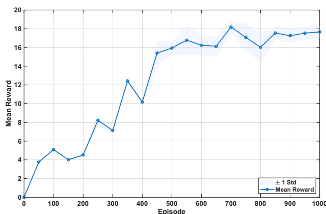
Figure 6: The convergence of RL in the HM3 at the architecture space.
