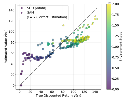
Figure 3: Scatter plot of estimating true returns V vs estimated returns \hat{V} . \hat{V} is closer to V when we use SAM as our base optimizer especially during the later env. steps.
