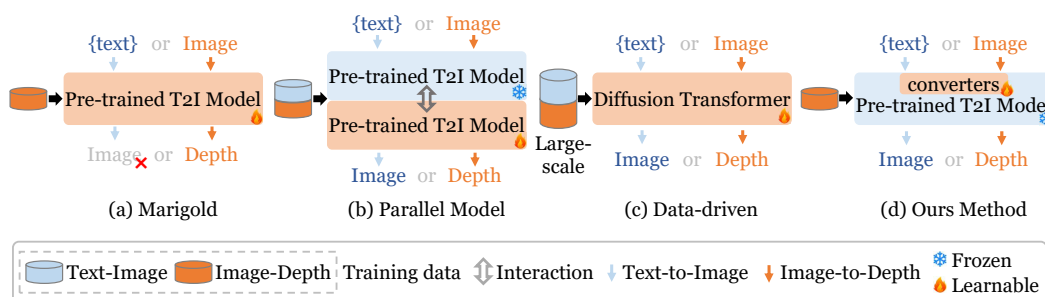
Figure 2: The comparison between existing methods and ours shows that, unlike previous works, our method requires only a few additional parameters to unleash its powerful depth estimation capability without compromising its inherent T2I generation ability.
