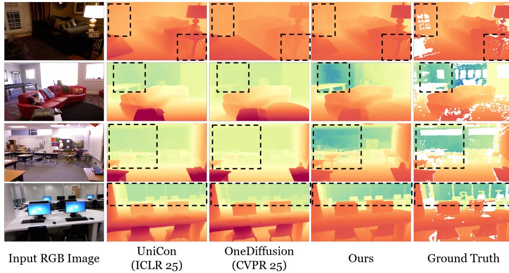
Figure 6: Qualitative comparison between MERGE and other unified image generation and depth estimation methods on the NYUv2 benchmark. MERGE shows better depth estimation results, especially in detailed areas (such as free-form voids and reflect regions).
