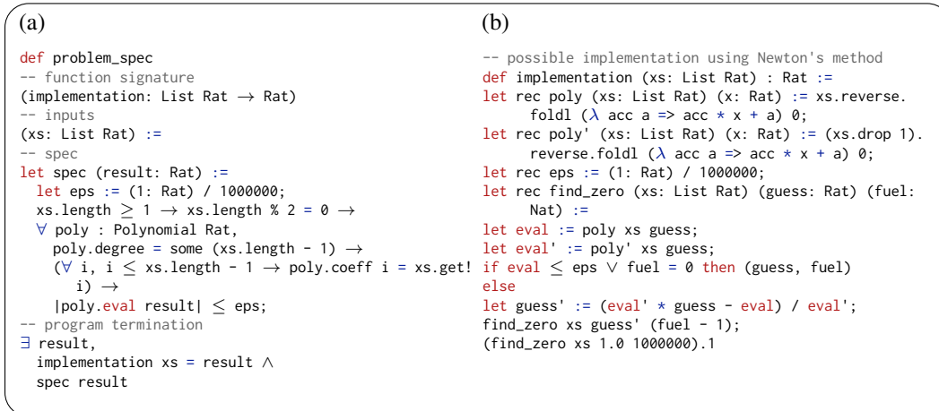
Figure 4: Polynomial Root-Finding. Problem 32 asks for an approximate real root of a degree- n polynomial. The spec enforces small residual error ( < 10^{-6} ). The implementation uses Newton’s method with bounded recursion; proving termination is non-trivial due to lack of guaranteed derivative behavior.
