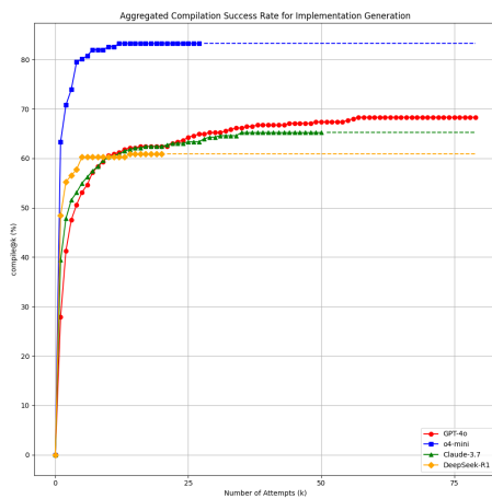
(c) Implementation Compilation (compile@k)
