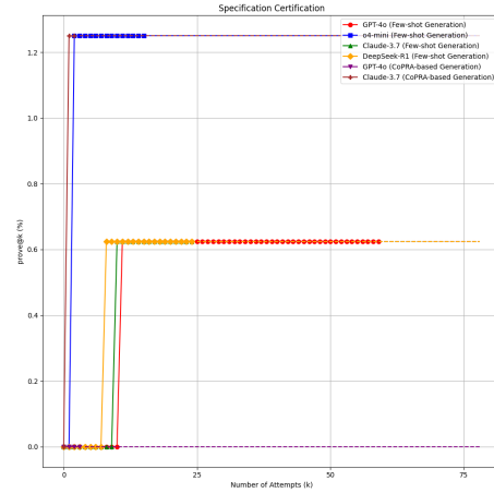
(b) Specification Certification (prove@k)
