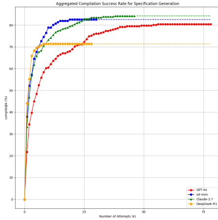
(a) Specification Compilation (compile@k)
