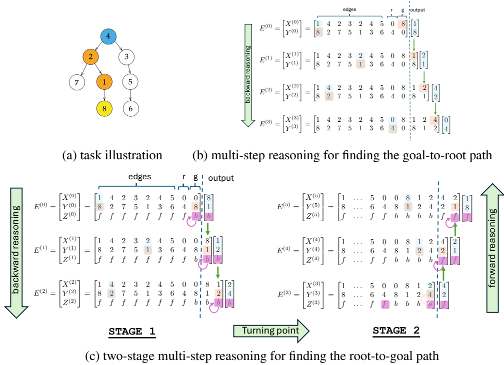
Figure 2: The multi-step reasoning process of the constructed transformers for the backward and forward reasoning tasks. Color indicates the attention association and output in each step.
