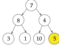
Figure 3: An example of a perfect binary tree of depth m = 2 and distinct nodes.
