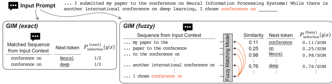
Figure 3: Overview of the GIM pipeline. GIM predicts the next token by efficiently searching for potential next-token completions in the input context with either exact or fuzzy matching.
