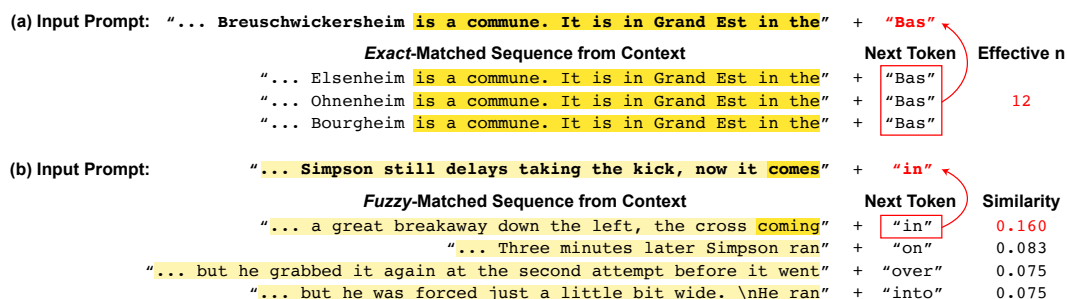
Figure 5: GIM's token-level attribution by tracing predictions to (a) exact or (b) fuzzy matches in prior context. Yellow highlight shows the match, and red box marks the source of the final prediction.
