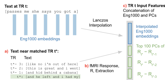
Figure 6: fMRI feature construction. (a) At each TR t , we retrieve a prior TR t^* with various matching methods. (b) We extract the top 100 principal components (PCs) of neural response changes before t^* . (c) These are concatenated to interpolated Eng1000 embeddings for fMRI signal prediction at TR t .
