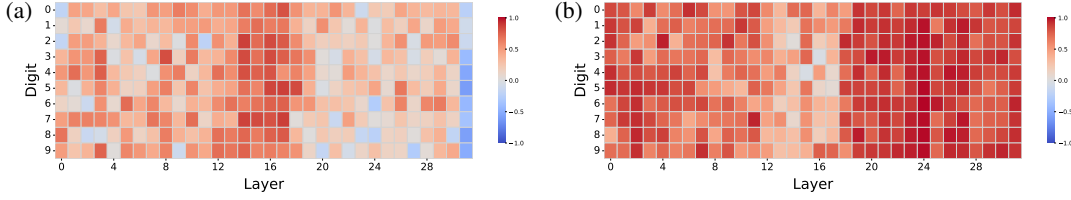
Figure 6: (a) Self-attention DSC vs. residual DSC. (b) FFN DSC vs. residual DSC. Self-attention exhibits moderate correlation in middle layers, while the FFN shows a stronger correlation in the later layers, highlighting the FFN’s role in driving digit bias.
