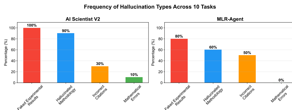
Figure 6: Frequency of each hallucination type in AI Scientist V2 and MLR-Agent across 10 tasks.
