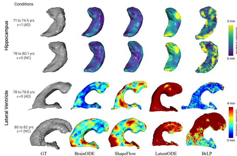
Figure 9: Qualitative results of 1-shot prediction for hippocampus and LV shapes. The color map indicates Euclidean distance errors (up to 2 mm for hippocampus, 4 mm for LV) between ground truth (GT) and predicted shapes.
