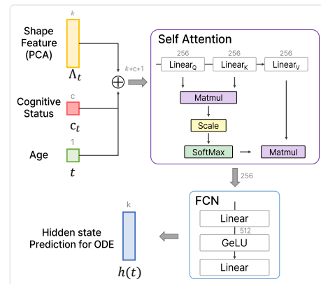
Figure 6: BrainODE architecture
