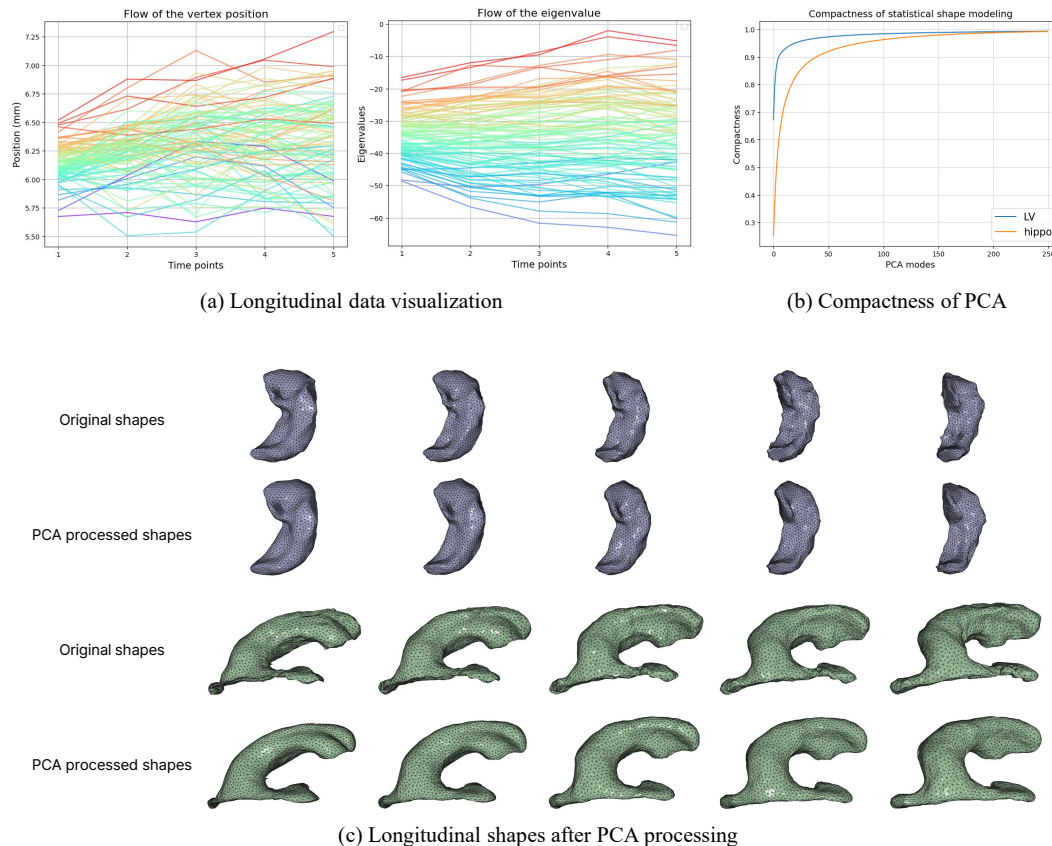
Figure 5: Impacts of shape dimensionality reduction using PCA. (a) Visualization of vertex positions and the first PCA eigenvalue across longitudinal observations from the LBC1936 dataset. (b) Compactness measures of hippocampus and LV across varying numbers of PCA modes. (c) Qualitative comparison between original shapes and their PCA-reconstructed shapes with 150 modes.
