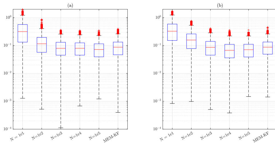
Figure 8: Location error for the localization tasks with unknown data association. (a) The underlying real association follows the same distribution in (17). (b) The measurement comes more from the landmarks at the lower left corner. We compare the 2-norm between the estimated position and the ground truth for all 100 trajectories. We compared the particle filters with N particles with the proposed MEM-KF with polynomial order up to r = 4 . We find that the particle filter with a sufficient number of particles and the proposed MEM-KF can estimate the trajectories with similar quality.
