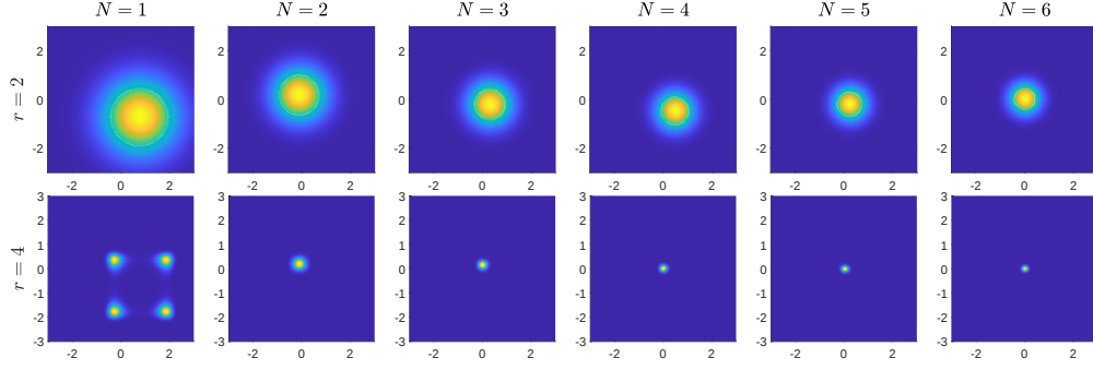
Figure 3: Applying the update step of MEM-KF to the linear system corrupted by noise (15). With larger r , the posterior distribution converges faster to the truth states. The case for noise (14) is presented in the Appendix.
