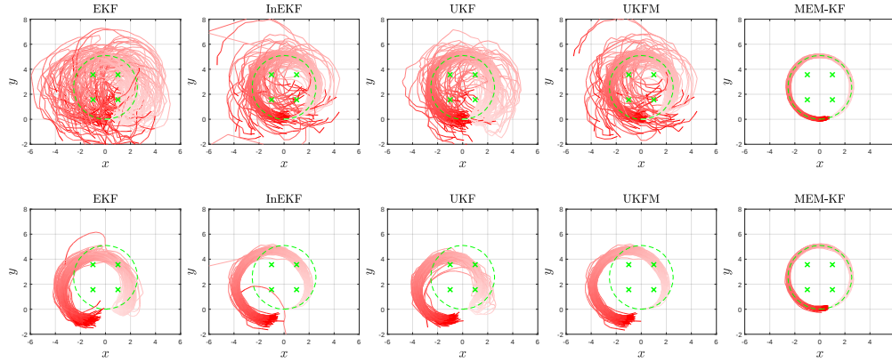
Figure 4: Localization with unknown data association. In the first row, the landmark association follows the same distribution in (17). In the second row, the measurement comes more from the landmarks at the lower left corner. The performance of baselines degrades due to incorrect data associations, while MEM-KF can consistently track the ground truth.
