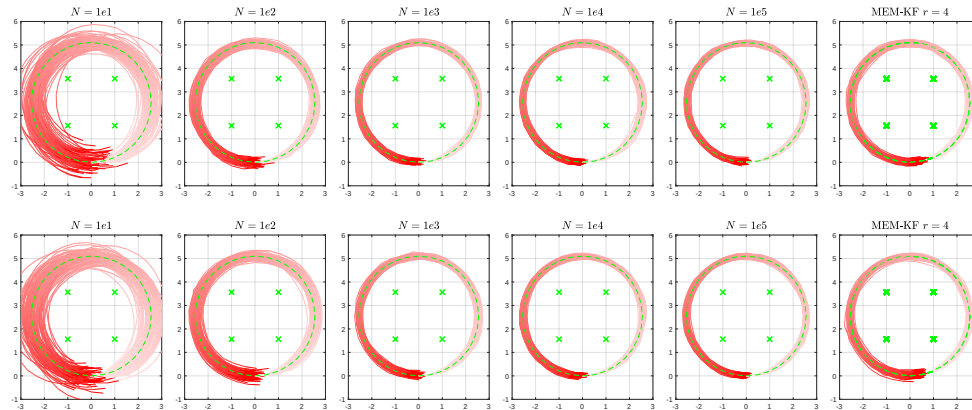
Figure 5: Comparison of particle filter with N particles with MEM-KF. In the first row, the landmark association follows the same distribution in (17). In the second row, the measurement comes more from the landmarks at the lower left corner. We see that the particle filter can better track the trajectories with more particles. We find that both the particle filter with a sufficient number of particles and MEM-KF can estimate the trajectories with similar quality. The statistics are presented in Figure 8.
