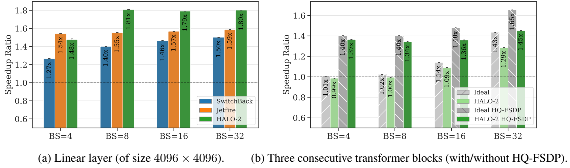
Figure 4: INT8 forward + backward speedups (over BF16) for 512 sequence length in LLAMA3-8B across batch sizes (BS). HALO-2 refers to HALO-2( \mathbf{F}^H, \mathbf{E}^H, \mathbf{G}^H ).
