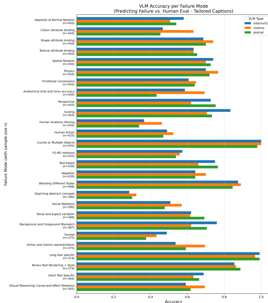
Figure 6: Comparison of VLM Accuracy Across Different Failure Modes. Accuracy is defined as the VLM's predicted failure boolean matching the human evaluation boolean for tailored captions. Average accuracy across all failure modes: Molmo-72B 76.5 \pm 1.5\% , InternVL3-78B 75.5 \pm 1.6\% , Pixtral-124B 74.2 \pm 1.6\% ( n=750 prompts per model). The three VLMs demonstrate comparable performance with no statistically significant differences in most pairwise comparisons.
