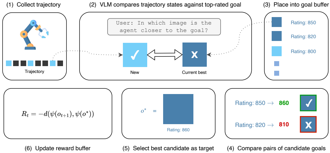
Figure 1: Summary of GoalLadder. (1-2) An agent collects a trajectory using the current SAC policy. Trajectory observations are uniformly sampled and compared against the current best candidate goal in the buffer. (3) If successful, they are placed into the candidate goal buffer. (4) Pairs of candidate goals are sampled and compared against each other using a VLM. Their ratings are updated after each comparison. (5-6) Periodically, the target state is updated with the current top-rated goal from the candidate buffer. Reward function is defined as the negative distance to the current best candidate goal in a learned embedding space; the RL agent is then trained with this reward. The process returns to step 1 and repeats.
