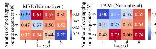
Figure 7: Comparison of the normalized MSE ( left ) and TAM ( right ) over different settings of the overlapping predictions N and the lag l . The x-axis represents the lag l , and the y-axis represents the number of overlapping predictions N . Increasing N improves TAM, while increasing l degrades the performance. No distinct tendencies are observed regarding MSE. Blue represents better performance.
