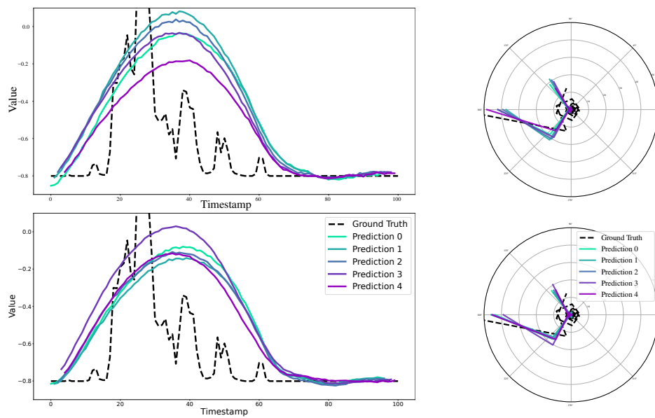
Figure 12: Visualization: Upper shows the prediction of iTransformer [30] using only the regression loss on the Solar dataset [24], while Bottom shows the result under the same conditions when AliO is also applied. It is observed that AliO improves alignment performance for overlapping timestamps.
