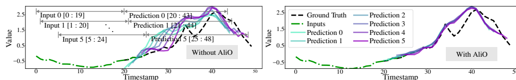
Figure 2: (Left) Six prediction outputs from the DLinear [40] model trained with regression loss (MSE) only, forecasting a length-24 sequence for ILI data [37], where six input sequences (green dotted line) are lagged one timestamp apart. (Right) Six predicted sequences from DLinear trained with AliO, under the same conditions. The predicted sequences exhibit improved output alignment, showing a closer match to the ground truth for all six predictions, which significantly reduces the prediction shifts observed when using regression loss alone.
