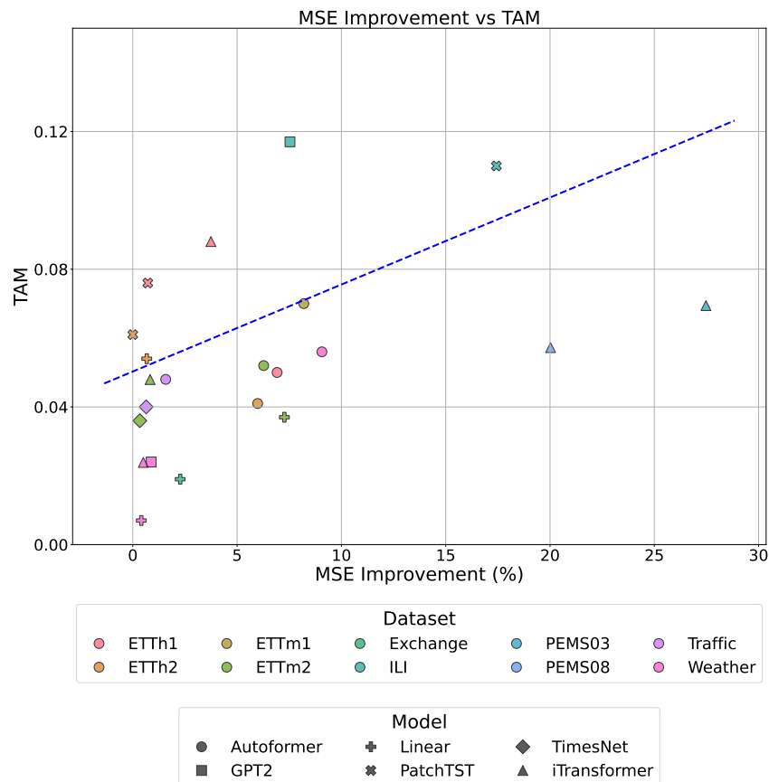
Figure 13: The relationship between initial TAM and MSE improvement (%).
