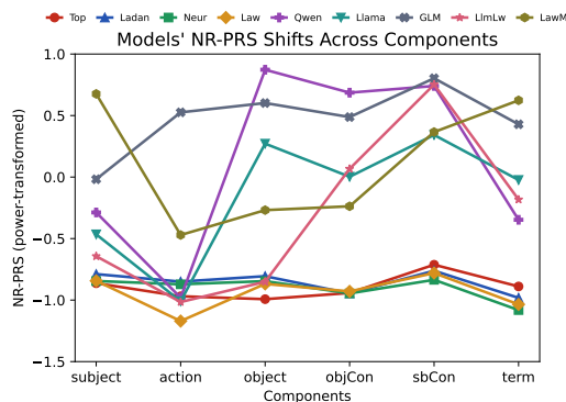
Figure 4: Relative pass rate shifts across components.
