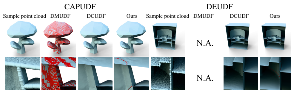
Figure 14: More results of non-manifold surface extraction from CAPUDF and DEUDF.
