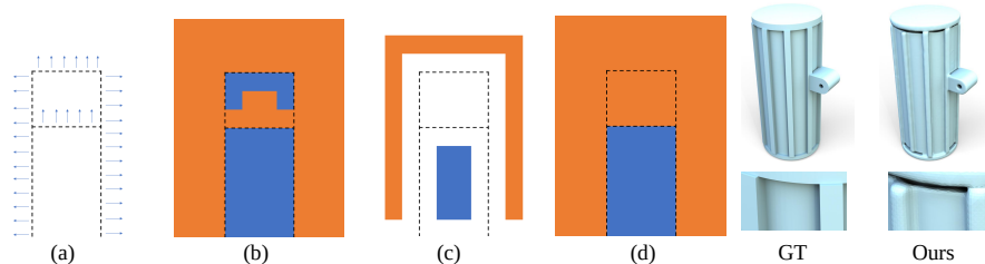
Figure 10: For a small MI region (upper part) (a), the inner voxels of its local two-signed field (b) will be removed during the erosion process, resulting in no seed region in the entire internal space (c). Consequently, the structure cannot be recovered after \alpha -expansion (d).
