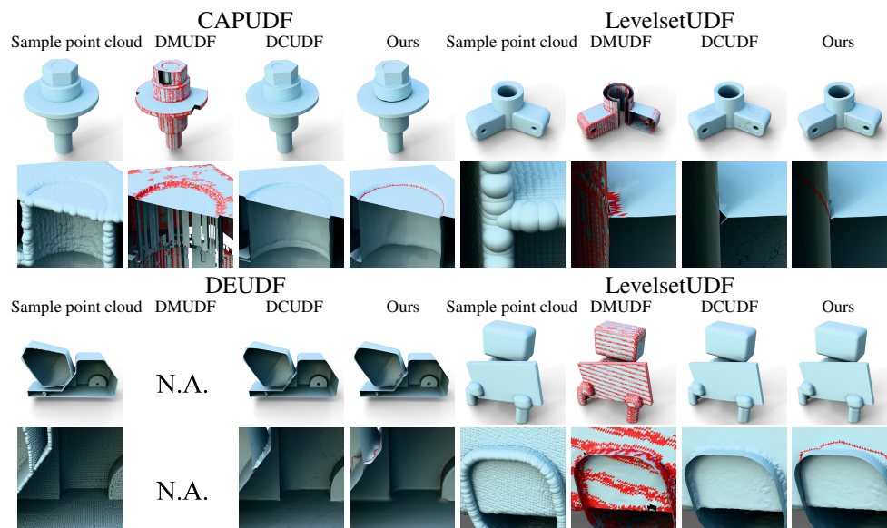
Figure 6: Non-manifold surface extraction from UDFs learned by CAPUDF [6], LevelSetUDF [7], and DEUDF [8]. We present the sampled point cloud on the UDFs as the GT (Ground Truth). We compare our surface extraction method with DCUDF and DMUDF, highlighting non-manifold edges in red in the results. While DMUDF frequently produces non-manifold edges in regions that should be manifold, DCUDF consistently generates double-layered manifold meshes, leading to a failure in preserving the correct topology of the target surfaces.
