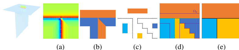
Figure 3: Illustration of global multi-labeled field generation from the local two-signed field on a T-shaped model. The close-up view of the cross-section on the non-manifold structure is provided. The local two-signed field w_S^l is first computed (a). Applying connected component labeling to the local two-signed field introduces artifacts due to small “tubes” (b). Erosion effectively removes these connected “tubes” (c). We solve the Equation 3 to fill the blank region (d). Comparing to dilate operation, it produce a more consistent boundary to the origin labeling (dash line). But our current result is over-segmented. We introduce an envelope \Omega_2 that is closer to the target surface than \Omega_1 . As shown in (e), the partition boundaries inside \Omega_2 is shown in green and outside in red. We merge two regions whose most adjacent boundaries are in red to get the final labeling result (e).
