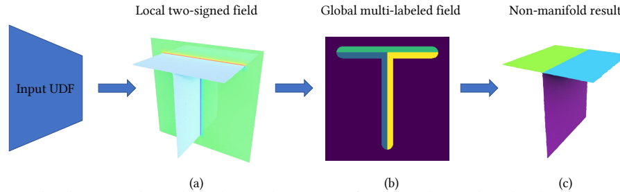
Figure 2: Pipeline: Starting with a learned UDF, we first sample a point cloud to compute a local two-signed field to differentiate the two sides of local manifold patches (a). We do not calculate regions far from the target face and label them as background (the green region in (a)). This is followed by generating a global multi-labeled field based on the two-signed field, which distinguishes all sides of the non-manifold surface (b). Finally, the non-manifold surface is extracted from the multi-labeled distance field using a multi-label MC algorithm (c).
