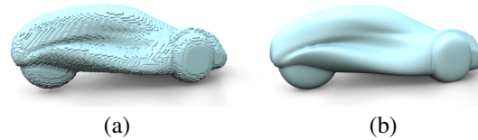
Figure 4: The Multi-Labeled Field computed from the point cloud, while having the correct topology, generates a noisy mesh because its zero level set is misaligned with the target surface (a). We use the input UDF to refine the result (b).
