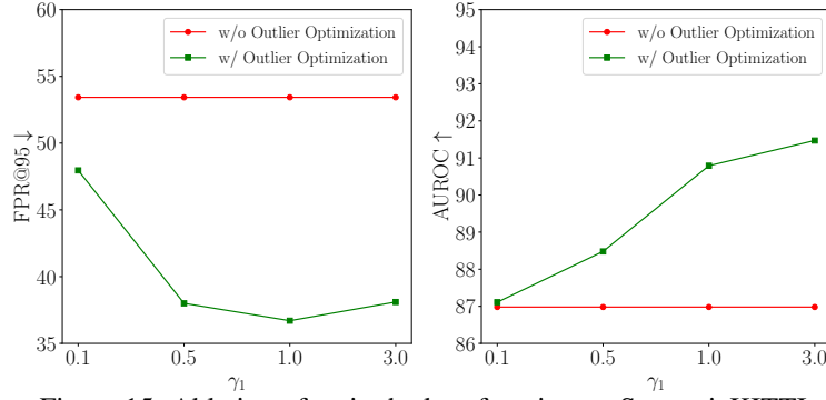
Figure 15: Ablation of \gamma_1 in the loss function on SemanticKITTI.
