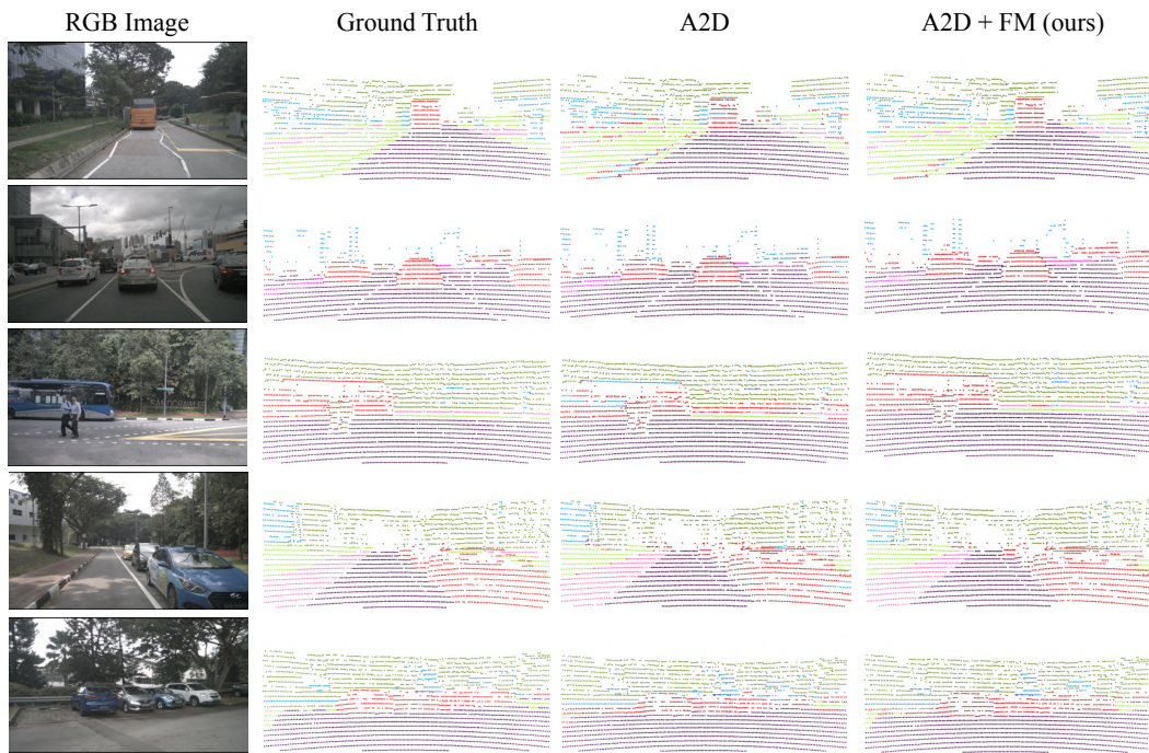
Figure 11: More visualizations on nuScenes dataset. Points with red color are OOD objects. Our method accurately segments OOD objects, outperforming the baseline method.
