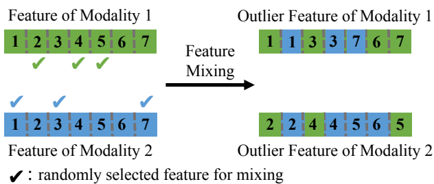
Figure 3: Illustration of Feature Mixing.
