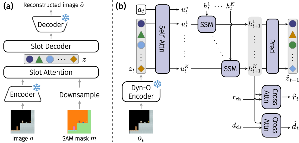
Figure 2: Components of Dyn-O: (a) object-centric representation learning; (b) dynamics learning. Modules marked with \text{✶} are fixed, while others are learnable. The "Dyn-O Encoder" in (b) corresponds to the lower half of (a), which maps the image o to the latent slot feature z . See Section 3 for details.
