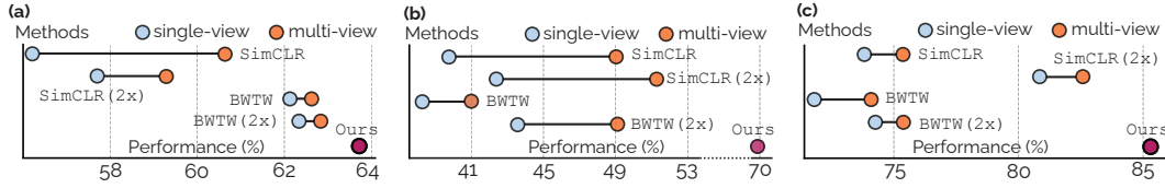
Figure 4: Performance comparison across datasets, (a) DaLiA ( \rho ), (b) HHAR (Acc), and (c) Chapman (F1), when adding a third view for instance discrimination similar to our method. While prior methods benefit from the additional view, their performance still lags behind our approach by a large margin.
