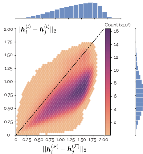
(c) Pairwise \ell_2 distance comparison between time and Fourier domain latent spaces on Sleep
