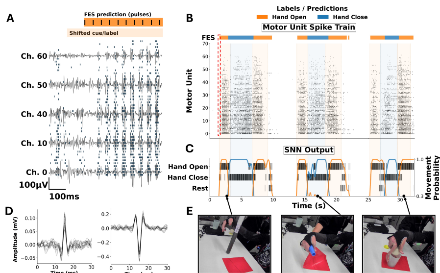
Figure 3: Spinal cord injury participant controls functional electrical stimulation (FES) in real-time via intention decoded from motor unit activity using a spiking neural network (SNN). A. Zoom-in plot of raw EMG with spike train on top at the transition between rest and hand open. Spikes are detectable in a 50ms window between FES pulses with 20Hz stimulation frequency. B. Full spike train that was decomposed in real-time while using the EMG-FES system in task practice. Rectangles above the spike train indicate the final movement predicted that triggered the corresponding FES movement to evoke assistance. The lighter shaded rectangles across the full spike train indicate the ground truth manually labeled by the operator. C. Output of the SNN with 3 classes and the resulting prediction probability based on the output neuron firing rates. D. Sample motor unit action potential waveforms averaged across the five highest weighted channels. E. Snapshots of SCI participant performing the rehabilitation tasks. See Supplementary Video 1 for a real-time demo.
