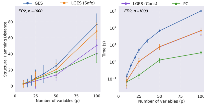
Figure D.1.4: Performance of algorithms on 50 simulated observational datasets from Erdős–Rényi graphs with p variables and 2p edges in expectation, given the smaller dataset of 10^3 samples and no prior knowledge (Sec D.1.5). In terms of accuracy, LGES (Conservative) outperforms other algorithms except for the case of p = 100 , when PC is more accurate.
