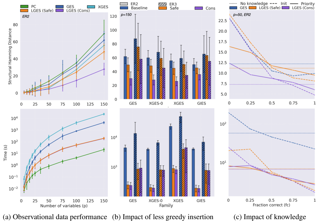
Figure 4: Performance of algorithms on 50 simulated datasets from Erdős–Rényi graphs with p variables. Lower is better (more accurate / faster) across all plots. (a) LGES outperforms baselines in accuracy and runtime on graphs with 2p edges in expectation, given n = 10^4 observational samples and no prior knowledge. (b) Less greedy insertion improves several GES variants on graphs with p = 150 variables and 2p and 3p edges in expectation, given n = 10^4 observational samples (and n = 10^3 samples per intervention for GIES) and no prior knowledge. LGES-0, LGES, LGES+, and LGIES are the less greedy variants of GES, XGES-0, XGES, and GIES respectively. (c) Given prior knowledge in the form of 3m/4 required edges when the true graph contains m edges, LGES' prioritization strategy is more robust to misspecification in the knowledge than initialization with the same knowledge, given n = 10^3 observational samples. See Sec. D for additional results.
