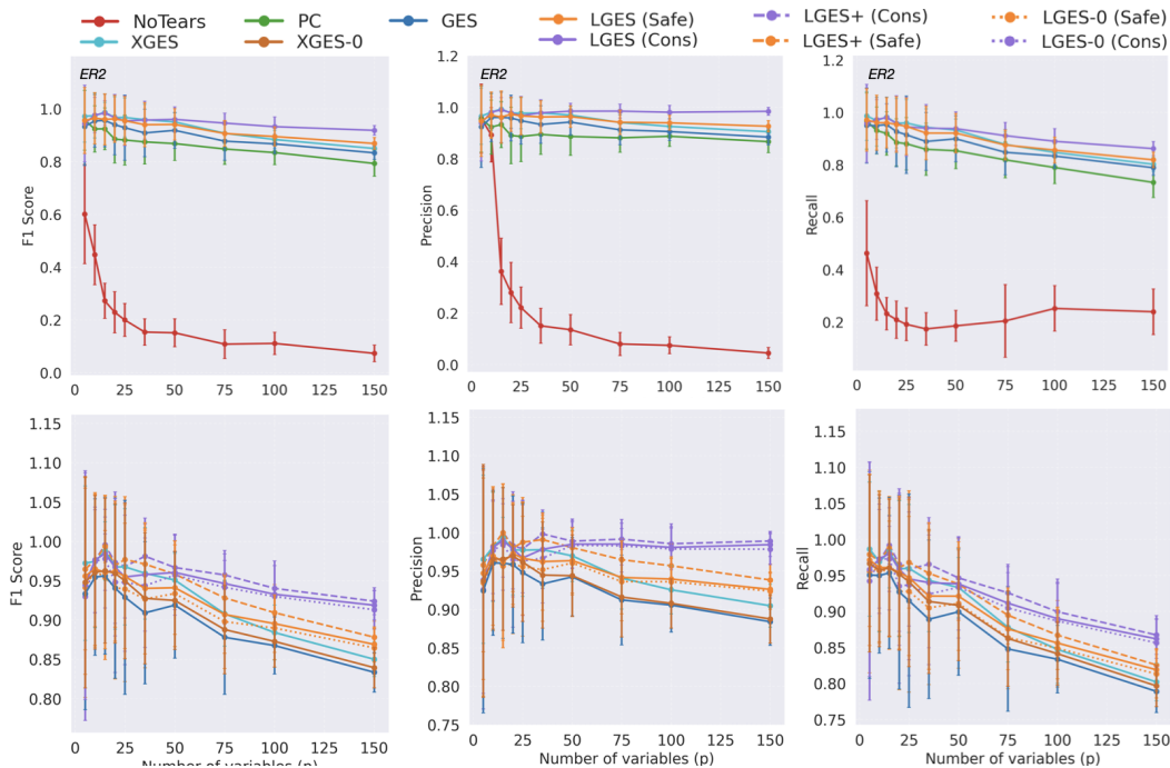
Figure D.1.2: Binary classification accuracy of algorithms on 50 simulated observational datasets from Erdős–Rényi graphs with p variables and 2p edges in expectation, given n = 10^4 samples and no prior knowledge (Sec. D.1.3). Higher is better across all plots. An MEC is said to contain an edge (X, Y) if it contains either X - Y or X \rightarrow Y (but not Y \rightarrow X ). (Top) Common baselines. GES-style algorithms outperform PC and NoTears in accuracy. (Bottom) GES variants. LGES-0, LGES, and LGES+ are the less greedy variants of GES, XGES-0, and XGES respectively. Each less greedy variant improves on its greedy counterpart in accuracy.
