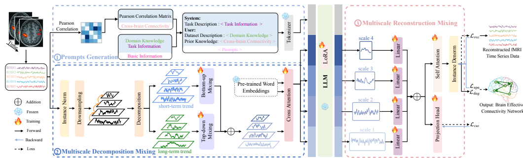
Figure 1: The overview of BrainEC-LLM framework. First, we enhance the inference capability of the LLM using ① prompts generation module. Next, we decomposition the complex variations in fMRI time series with ② multiscale decomposition mixing module, aligning pre-training word information of LLM with fMRI time series data. Finally, the multiscale features produced by LLM are combined across different scales using ③ multiscale reconstruction mixing module.
