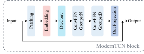
Figure 2: The architecture of ModernTCN block.
