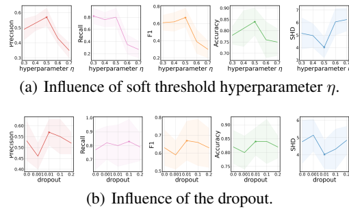
Figure 5: Hyperparameter analysis on the Smith dataset (the starred results are the best results).
