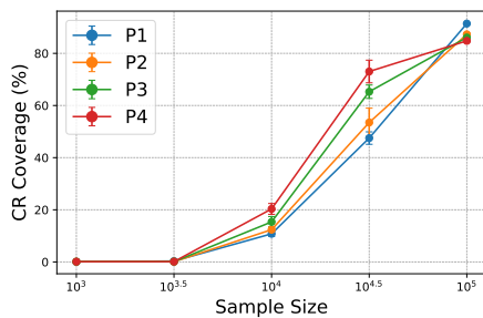
Figure 3: Percentage of real data samples that fall within the DiT-generated 95% CR.
