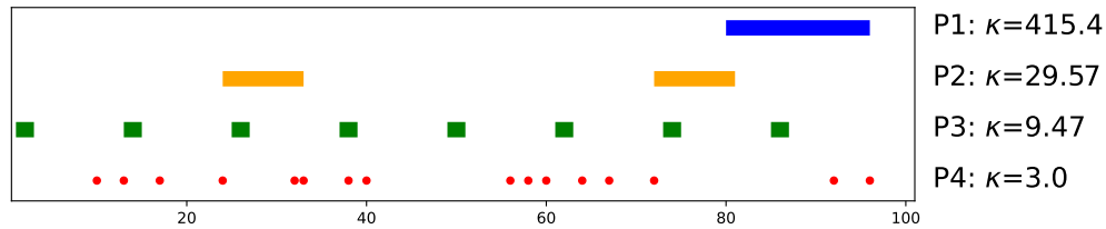
Figure 2: Visualization of the four missing patterns for a sequence of length 96. Each horizontal line shows the positions of missing values (highlighted in blue, orange, green and red for Patterns 1-4), and annotations on the right indicate the pattern number and its condition number \kappa(\Sigma_{\text{cond}}) .
