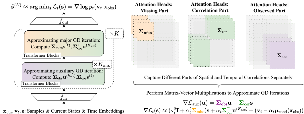
Figure 1: Constructed transformer architecture: Within each transformer block, attention heads focus on capturing information of different covariance components ( \Sigma_{\text{obs}}, \Sigma_{\text{cor}}, \Sigma_{\text{miss}} ) separately, and approximate corresponding matrix–vector multiplications. A total of K block groups perform major GD steps, with K_{\text{aux}} inner blocks in each group dedicated to solving the auxiliary problem.
