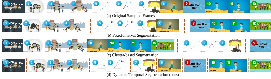
Figure 3: Visualization of different segmentation methods on 12 sampled frames from a video example. (b) Fixed-interval Segmentation struggles to maintain high intra-segment similarity, leading to visually diverse frames within the same segment. (c) Cluster-based Segmentation disrupts temporal order, grouping frames from different time periods to the same segment. (d) Our DySeg adaptively partitions the video, preserving both temporal structure and high intra-segment similarity. Please refer to Table 8 for a detailed quantitative comparison.
