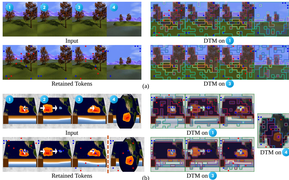
Figure 5: Visualization of FastVID with c = 0, \tau = 0.9, d = 0.4, p = 2 . We retain a total of 40 tokens, including 16 tokens in DTM (highlighted in red) and 24 in ATS (highlighted in blue). In DTM, patches that share the same inner and border color are merged.
