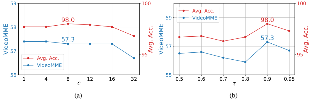
Figure 6: Ablation study on c and \tau in DySeg. c denotes the minimum number of segments in a video, whereas \tau denotes the transition similarity threshold. Both parameters jointly control the segmentation granularity.
