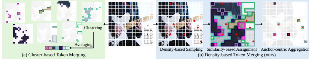
Figure 4: Comparison of our proposed DTM and Cluster-based Token Merging. (a) Cluster-based methods aggregate tokens within each cluster and concatenate them, leading to a loss of positional information and disruption of the spatiotemporal structure in video data. (b) Our DTM updates anchor tokens while preserving their original positional information, maintaining structural coherence. Please refer to Table 7 for a detailed quantitative comparison.
