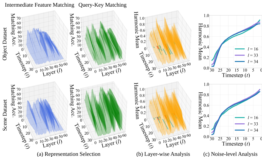
Figure A.2: Analysis of temporal matching in HunyuanVideo [49]. (a) Representation selection : Query-key matching achieves higher accuracy than intermediate feature matching. (b) Layer-wise analysis : Temporal correspondence is primarily governed by a limited set of layers. (c) Noise-level analysis : Temporal matching improves as noise decreases.
