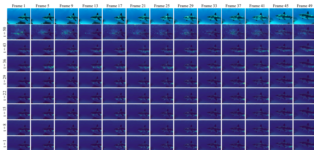
Figure A.19: Text-to-frame attention visualization for the word “shark” across denoising timesteps at layer l = 17 . Attention evolves from coarse to fine throughout denoising ( t = 50 to 1 ), indicating that the text prompt primarily guides the global semantic layout in early timesteps.
