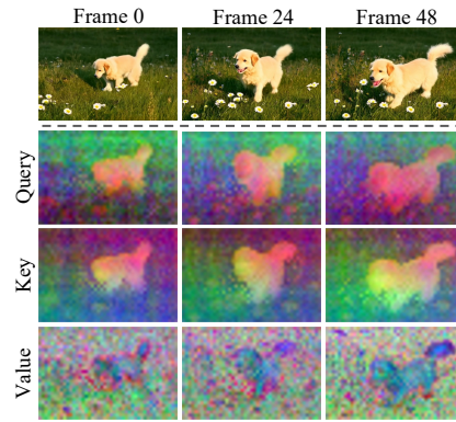
Figure A.7: PCA visualization of queries, keys and values.
