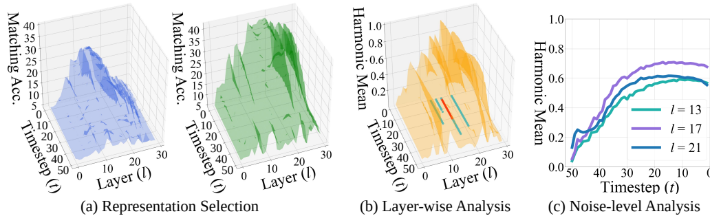
Figure A.5: Analysis of temporal matching in CogVideoX-2B [84] with DAVIS [19] dataset. (a) Representation selection : Query-key matching achieves higher accuracy than intermediate feature matching. (b) Layer-wise analysis : Temporal correspondence is primarily governed by a limited set of layers. (c) Noise-level analysis : Temporal matching improves throughout the denoising process and slightly degrades near the end.
