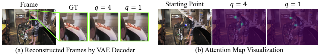
Figure A.10: Analysis of temporal compression. (a) Reconstructed frames from the VAE decoder using different temporal compression ratios q . (b) Visualization of attention maps under different temporal compression ratios.
