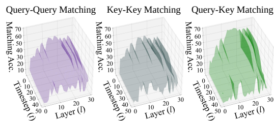
Figure A.8: Comparison of query-query, key-key, and query-key matching.
