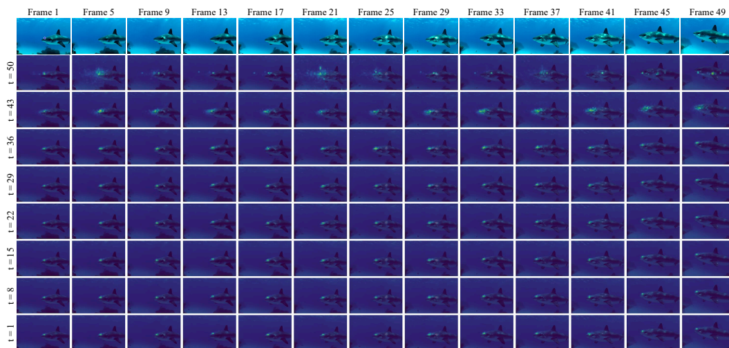
Figure A.18: Cross-frame attention visualization across denoising timesteps at layer l = 17 . Attention progressively sharpens and localizes throughout denoising ( t = 50 to 1 ).
