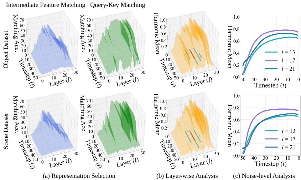
Figure 4: Analysis of temporal matching in CogVideoX-2B [84]. (a) Query-key matching outperforms intermediate feature matching, highlighting the effectiveness of cross-frame interactions in 3D attention. (b) The harmonic mean of query-key matching shows that temporal matching is primarily driven by a few specific layers. (c) Temporal matching improves progressively during the denoising but slightly degrades near the final steps.
