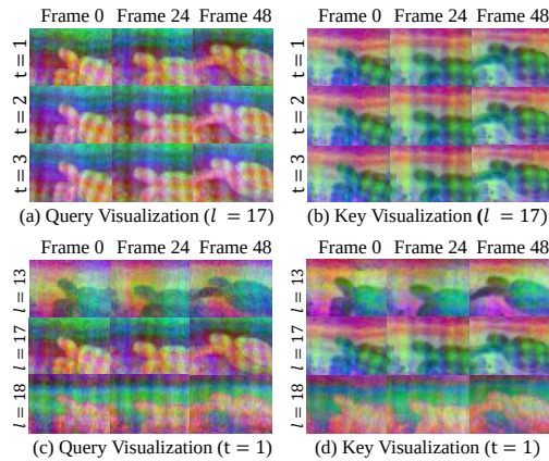
Figure A.9: PCA visualizations of query-key features across timesteps and layers.
