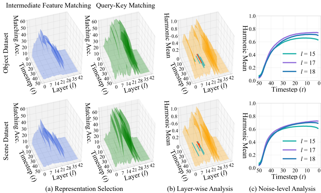
Figure A.1: Analysis of temporal matching in CogVideoX-5B [84]. (a) Representation selection : Query-key matching achieves higher accuracy than intermediate feature matching. (b) Layer-wise analysis : Temporal correspondence is primarily governed by a limited set of layers. (c) Noise-level analysis : Temporal matching improves as noise decreases but slightly degrades near the final steps.
