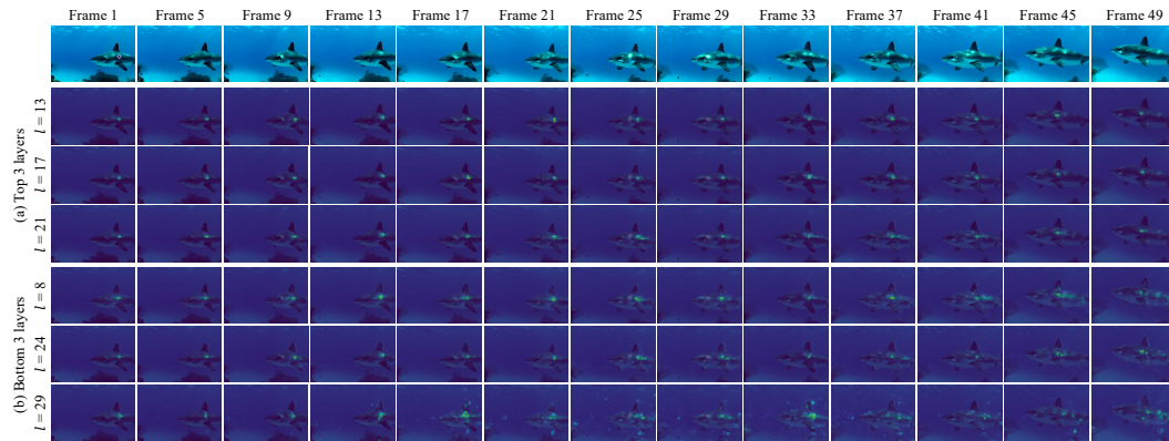
Figure A.17: Cross-frame attention visualization across layers at timestep t = 1 . (a) Top-3 layers ( l = 13, 17, 21 ) exhibit sharp and precise localization. (b) Bottom-3 layers ( l = 8, 24, 29 ) display diffuse and scattered attention.
