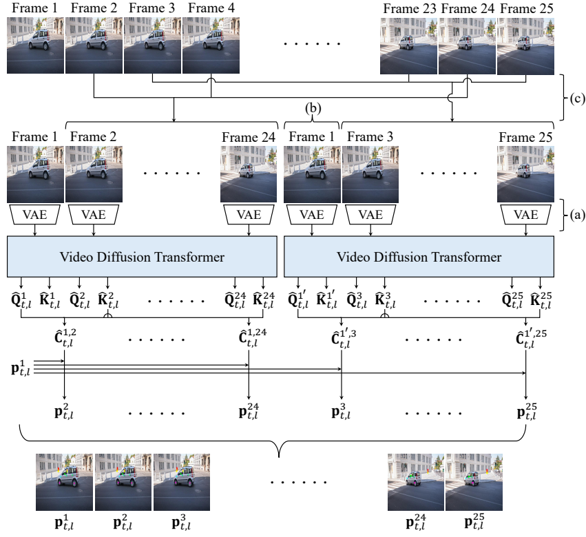
Figure A.4: Overall architecture of DiffTrack for zero-shot point tracking. (a) Removing temporal compression improves point accuracy by avoiding interpolation. (b) A global first-frame is inserted into each chunk for direct matching. (c) Interleaved chunk construction reduces the temporal gap to the first frame.
