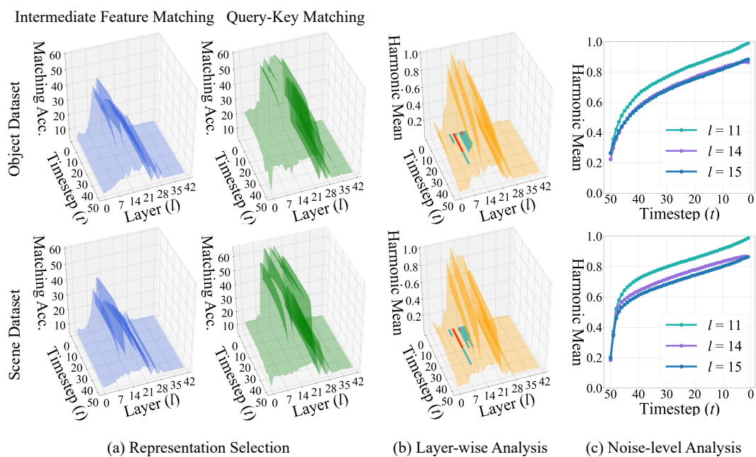
Figure A.3: Analysis of temporal matching in CogVideoX-5B-I2V [84]. (a) Representation selection : Query-key matching achieves higher accuracy than intermediate feature matching. (b) Layer-wise analysis : Temporal correspondence is primarily governed by a limited set of layers. (c) Noise-level analysis : Temporal matching improves during denoising steps.
