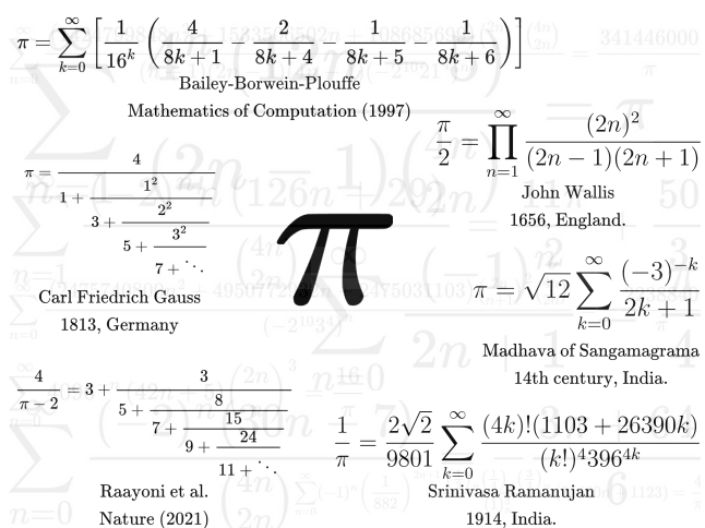
Figure 1: Selected \pi formulas across centuries.
