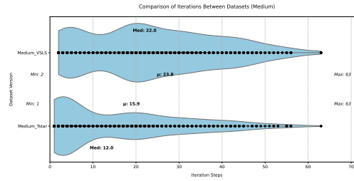
Figure 7: The comparative visualization of iteration counts on the medium-length video subset of the VIDEO-MME dataset demonstrates that our method consistently requires a higher number of iterations compared to the T* approach.
