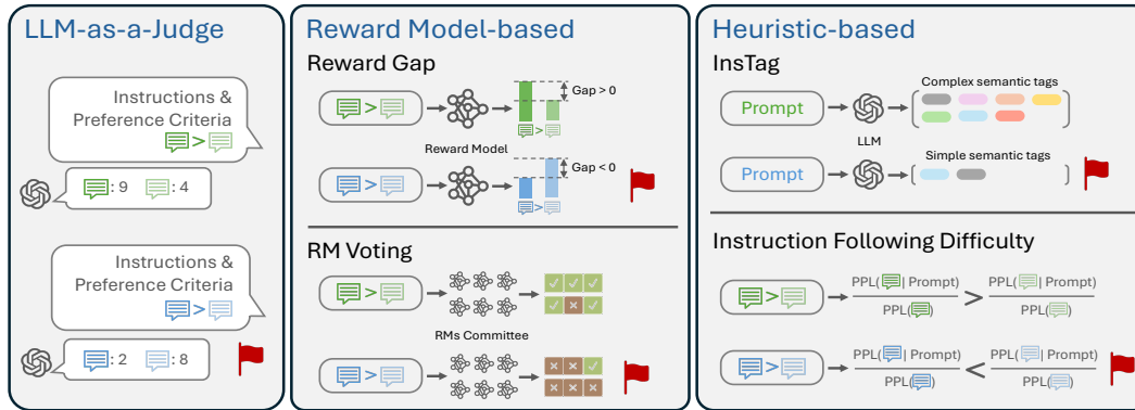
Figure 2: The summarization of data cleaning approaches for LLM alignment. We categorize data cleaning approaches into three groups based on the definition of unreliability they considered. The three groups include LLM-as-a-judge, score of reward model, and heuristic criteria. 🚩 indicates unreliable data identified by each approach.
