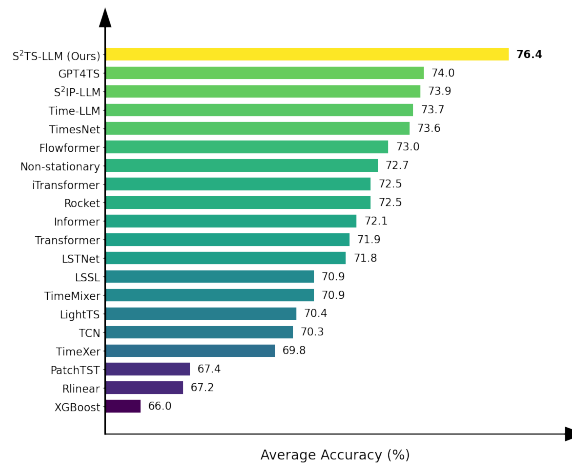
Figure 5: Classification results. The results are averaged from ten datasets of UEA. Detailed results are provided in Appendix E.5.
