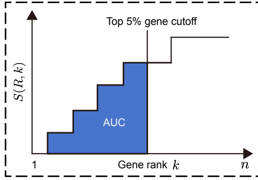
Figure 7: The recovery curve in the AUCell algorithm, with the gene ranking as x-axis and the recovery score as the y-axis.
